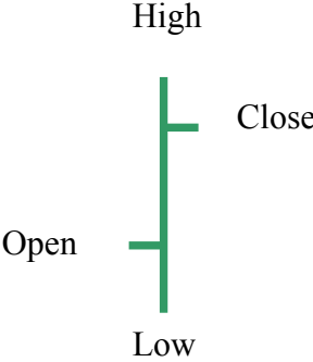
Bullish Bar
