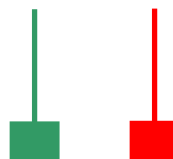
Shooting Star
