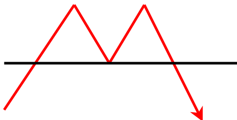
Double Top
