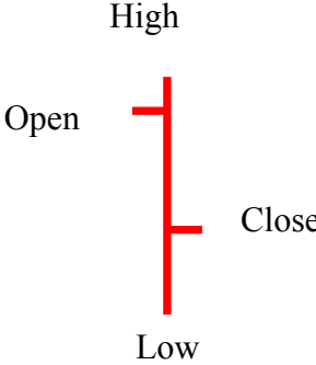
Bearish Bar
