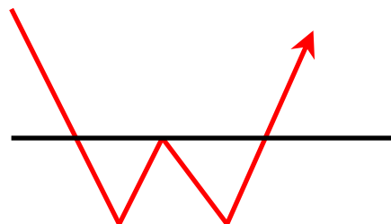
Double Bottom
