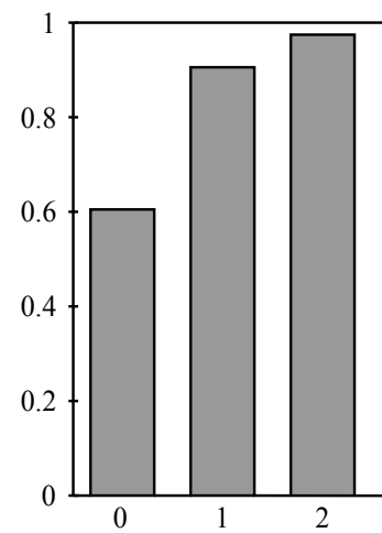
Figure B-11 Cumulative probability functions for the Poisson Distribution (L = .5).
