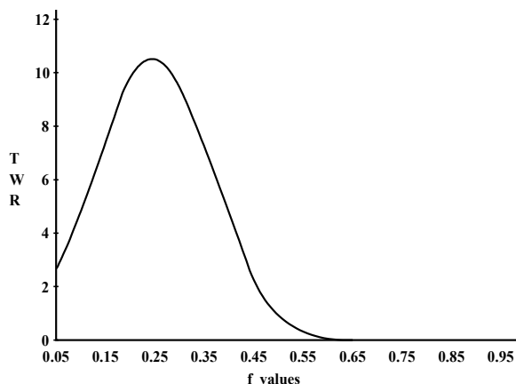
Figure 1-1 20 sequences of +2, -1.
