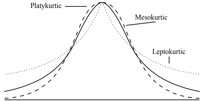
Figure 3-4 Kurtosis.
