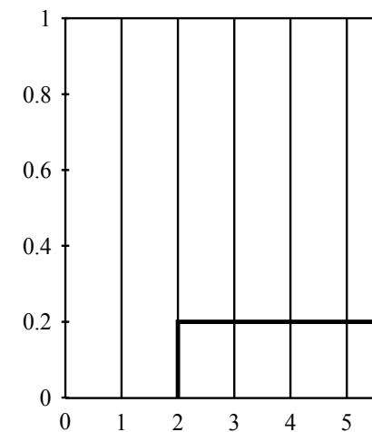
Figure B-1 Probability density functions for the Uniform Distribution ( A = 2, B = 7 ).
