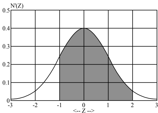
Figure 3-12 The area between -1 and +2 standard units.
