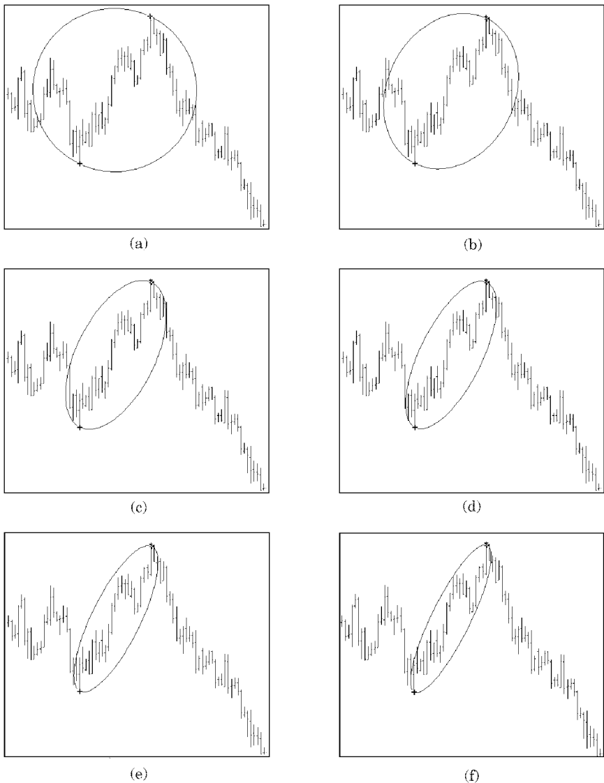
Figure 5.1 Generation of PHI-ellipses using different ratios from the PHI series. From top left to bottom right: ratio 1,000 (circle); ratio 1.618; ratio 4.236; ratio 6.854; ratio 11.090; ratio 17.944.
